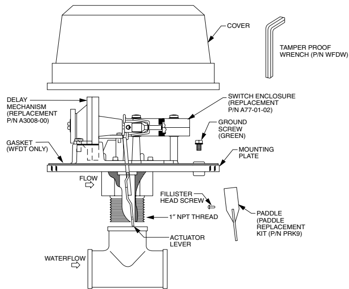
Figure 2. Assembly diagram:
