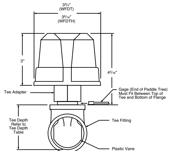
Figure 1. Mounting dimensions:
