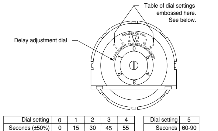
Figure 4. Delay adjustment dial:
