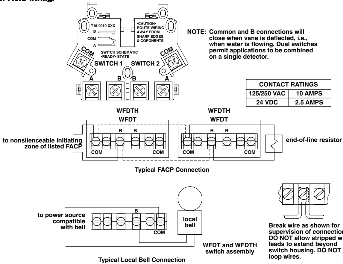
Figure 3. Field wiring:
