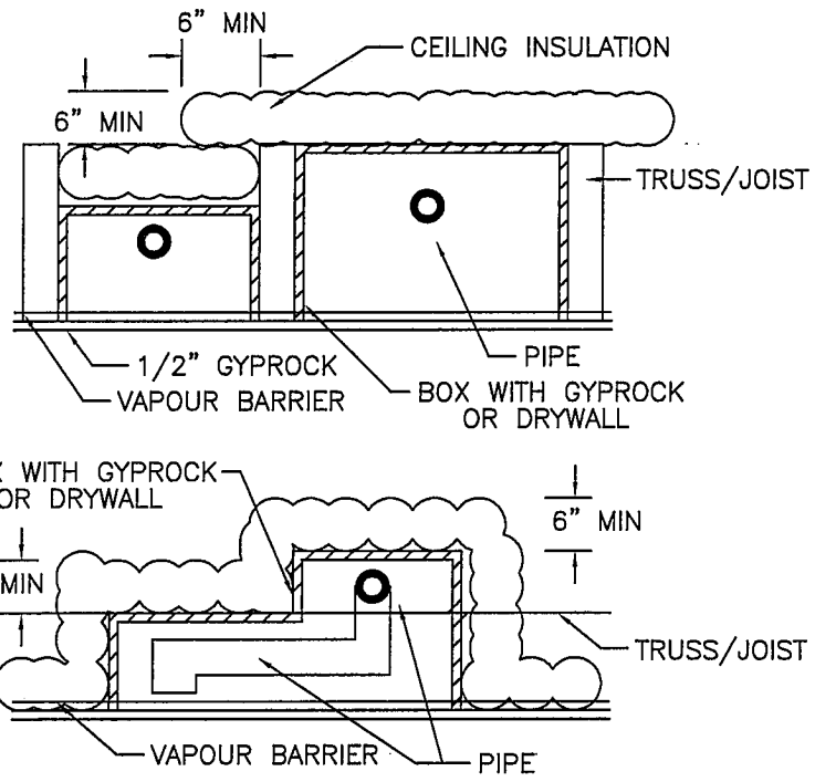
VANCOUVER INSULATION DETAIL N.T.S.
